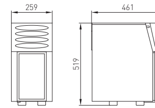
Under-counter cooling unit
