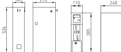
Coin changer Opens to the side (274 mm)
