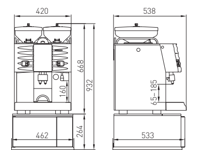
Under-machine cooling unit
