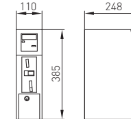
Coin changer Opens to the front
