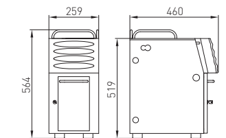
Flavour Point
