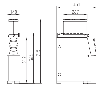
Powder system
