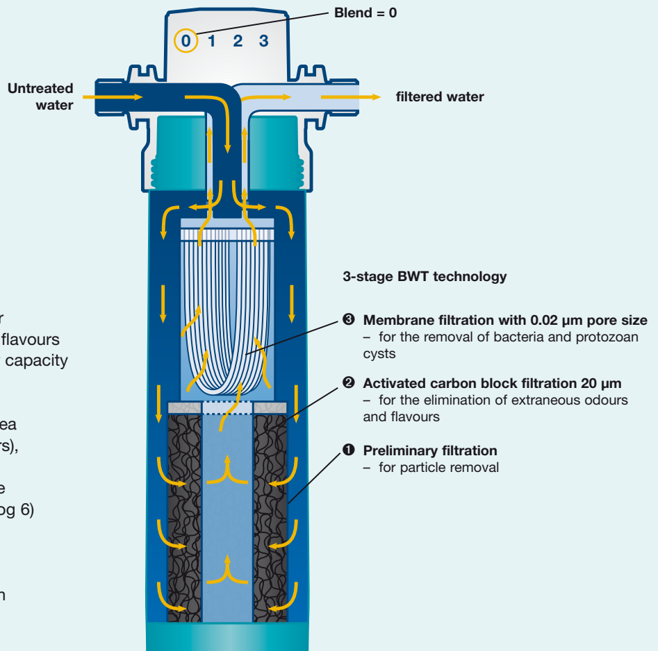
Structure of a BWT bestcare filter cartridge with 3-level filtration
